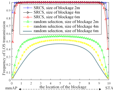
(a) SRCS algorithm
