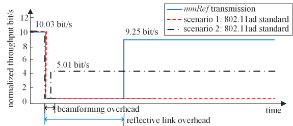
Fig. 9. The comparison of normalized transmission throughput.
