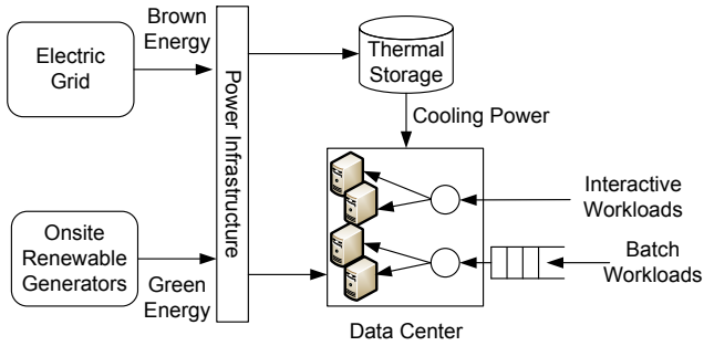
Fig. 1. Block diagram for system model
